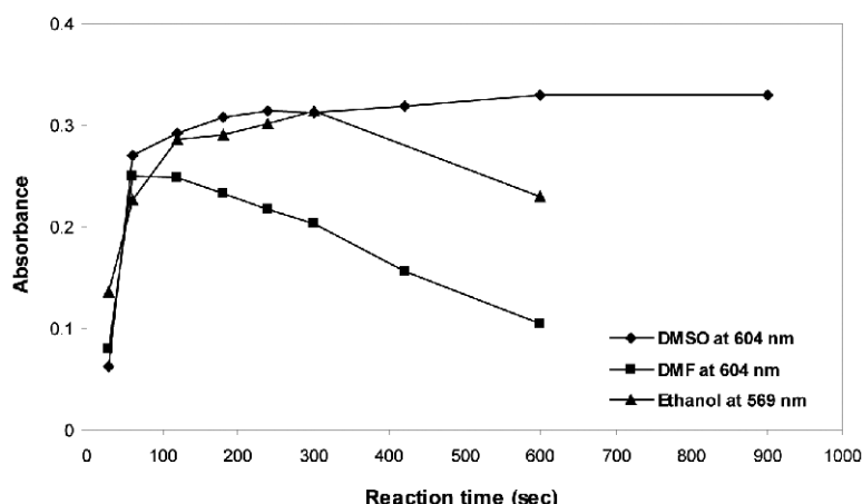
Figure 6. Stability of PAMAM G2 (fixed 371 nmol \text{NH}_2 ) reacted with ninhydrin in different solvents over different reaction time periods (average of two independent measurements).
