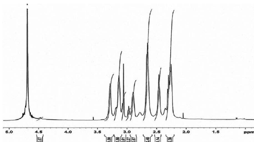
Figure 9. ^1\text{H-NMR} spectrum of QG4 in \text{D}_2\text{O} .
